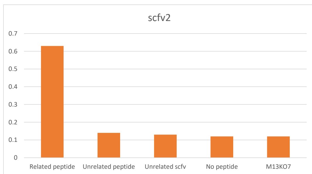
Fig. 6. Phage ELISA results of scFv2 (OD at 405 nm).
