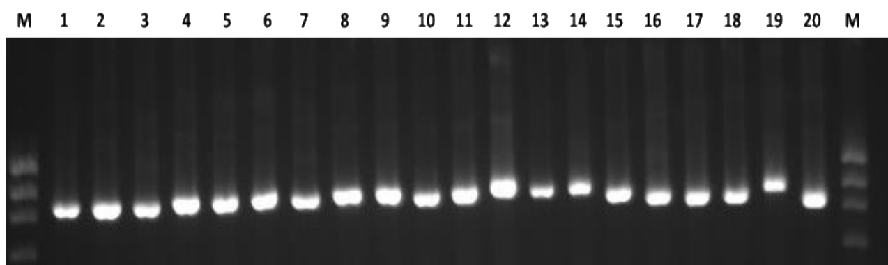
Fig. 3. PCR result of the selected clones after panning. 950 bp band was obtained. M: X174 DNA marker.
