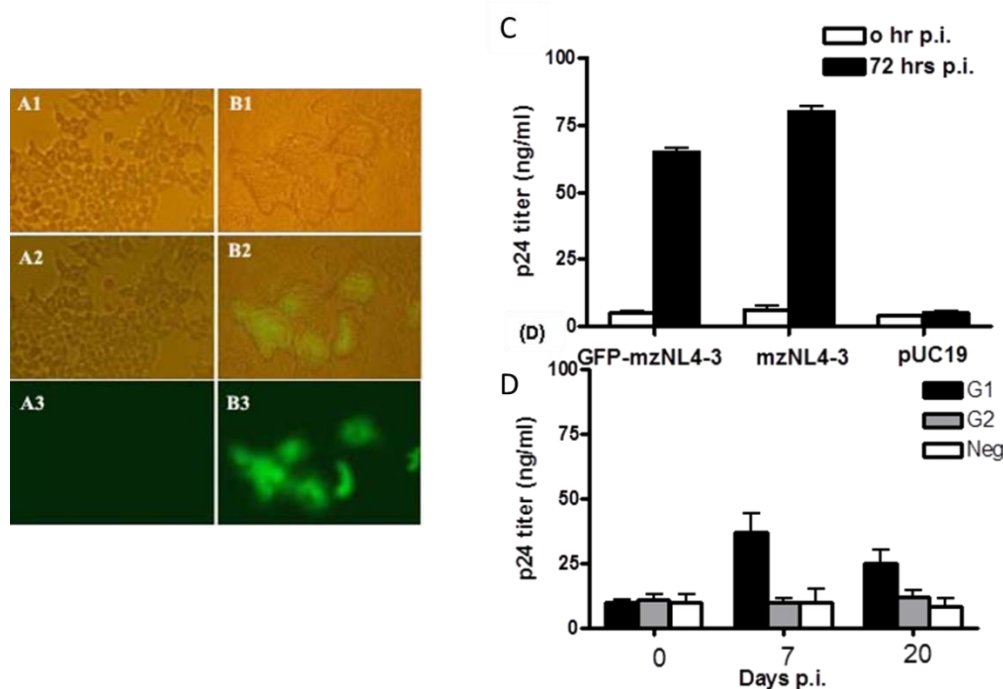
Fig. 3. Production of the second generation GFP-mzNL4-3 virions. 72 hrs post-infection (p.i.) HEK293T cells infected with the first generation GFP-mzNL4-3 virions (50 \mu g of p24) produced syncytium and showed GFP emission ( B1-B3 ), in contrast to control cells treated with the supernatant of pUC19-transfected cells ( A1-A3 ). GFP-mzNL4-3 infection (0.5 \mu g of p24) resulted in the secretion of p24 antigen as efficient as infection with mzNL4-3 virions ( C ). Cells infected with 0.5 \mu g of either the first generation (G1) or the second generation (G2) GFP-mzNL4-3 virions were assayed for p24 production up to 20 days p.i. Contrary to G1, the amount of measured p24 for G2 infected cells was not higher than that for non-infected control cells (Neg) in different time points. Bars represent mean of p24 concentration \pm SD in three infected wells ( D ).
