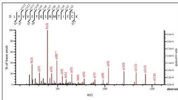
Fig. 4. MS/MS spectra of fragmented peptides derived from trypsin-digested rTrx-PD-L1.
