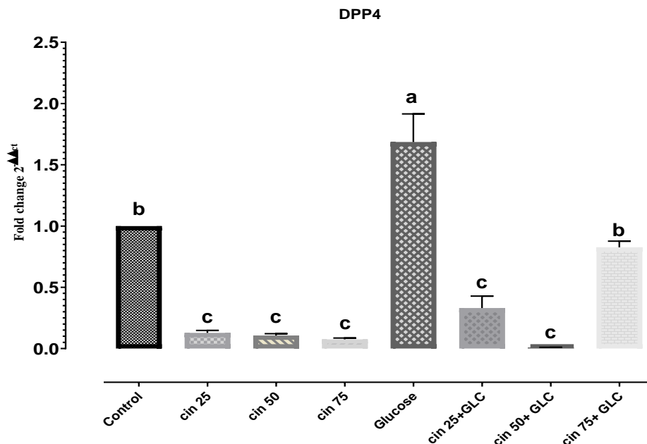
Fig. 7. Impact of different concentrations of cinnamic acid on the DPP4 gene expression in HepG2 cells after 48 hours treatment in the presence or absence of 60 mM of glucose. The findings are presented as Fold change 2^{-\Delta\Delta Ct} compared to the control group. Different letters in each column indicate a significant difference between groups.
