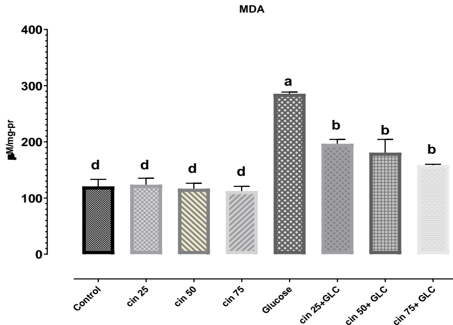
Fig. 6. Impact of different concentrations of cinnamic acid on the MDA protein in HepG2 cells after 48 hours treatment in the presence or absence of 60 mM of glucose. The findings are presented as \mu\text{M/mg} protein and are calculated as the mean (standard deviation) of three separate measurements. Different letters in each column indicate a significant difference between groups.
