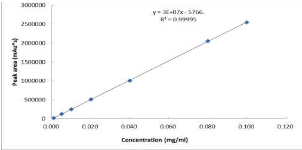
Fig. 2. The calibration curve of Orcinol - β - D - glucoside in HPLC fingerprinting: The signal E+7 means 10 7 .
